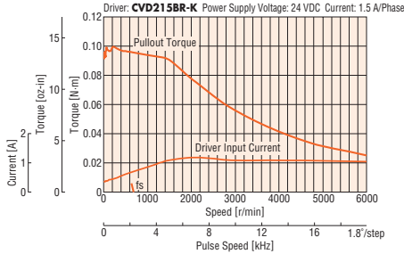
PKP223D15A2/ PKP223D15B2
