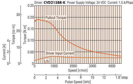
PKP225D15A2/ PKP225D15B2
