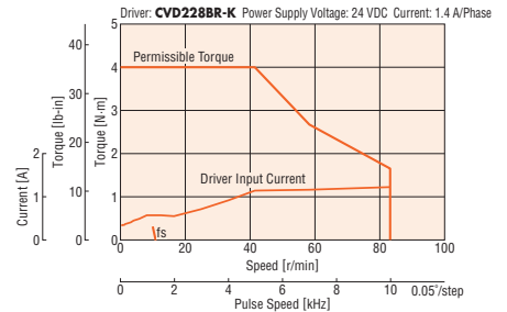
PKP264D14A2-SG36/PKP264D14B2-SG36
