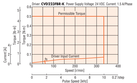
PKP243D15A2-SG9/ PKP243D15B2-SG9
