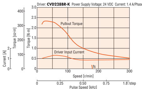
PKP268D14A2/PKP268D14B2
