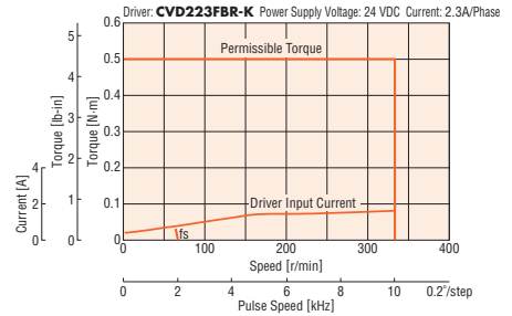
PKP243D23A2-SG36/PKP243D23B2-SG36
