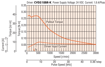
PKP544MN18A/PKP544MN18B
