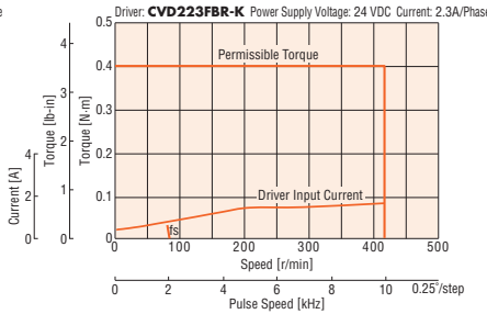
PKP243D23A2-SG18/PKP243D23B2-SG18
