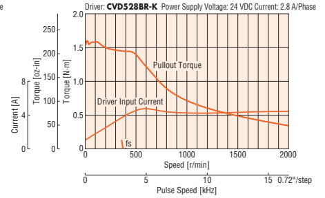
PKP568N28AA2/ PKP568N28BA2
