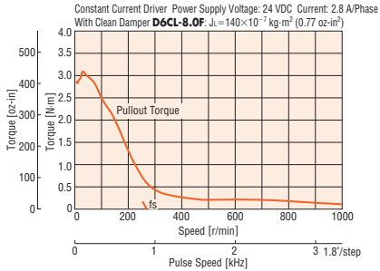
PV269-D2.8AA/PV269-D2.8BA
