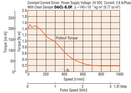
PV266-D2.8AA/PV266-D2.8BA
