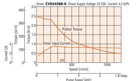
PKP268D42A2/PKP268D42B2
