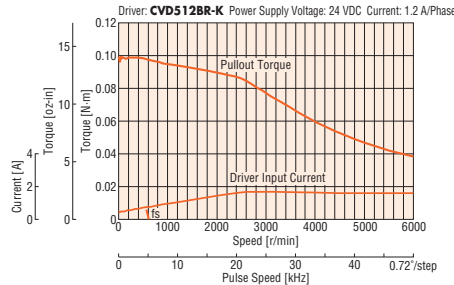
PKP525N12A/PKP525N12B
