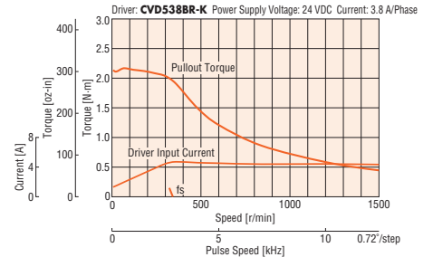
PKP569FN38A2/ PKP569FN38B2
