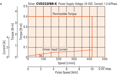
PKP243D15A2-SG7.2-R2FL
