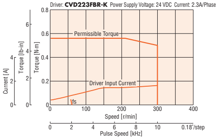
PKP243D23A2-SG10/PKP243D23B2-SG10
